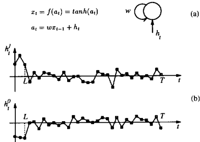
Fig. 1. (a) Latching recurrent neuron. (b) Sample input to the recurrent neuron. The trainable values (marked in bold) have been tuned by one of the successful learning simulations.
